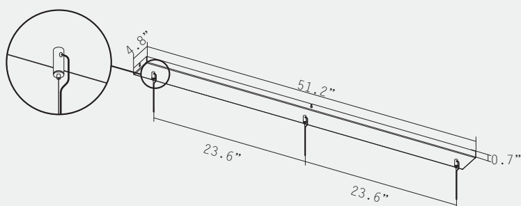
SPOT 6 CANOPY - SUSPENSION WIRE
